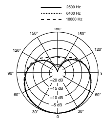
MX150/C Polar Pattern
