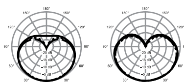
Legend for MX185: - 250 Hz (solid line) - 500 Hz (dashed line) - 1000 Hz (dotted line) - 2500 Hz (dash-dot line) - 6400 Hz (long-dashed line) - 10000 Hz (short-dashed line)
