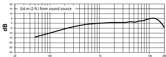
MX150/C Frequency Response
