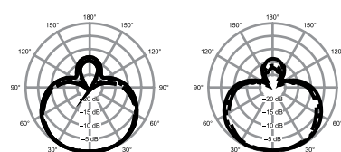
Legend for MX184: - 250 Hz (solid line) - 500 Hz (dashed line) - 1000 Hz (dotted line) - 2500 Hz (dash-dot line) - 6400 Hz (long-dashed line) - 10000 Hz (short-dashed line)
