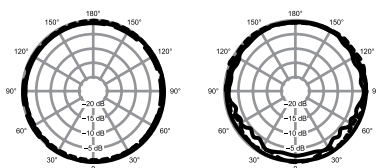
Legend for MX183: - 250 Hz (solid line) - 500 Hz (dashed line) - 1000 Hz (dotted line) - 2500 Hz (dash-dot line) - 6400 Hz (long-dashed line) - 10000 Hz (short-dashed line)
